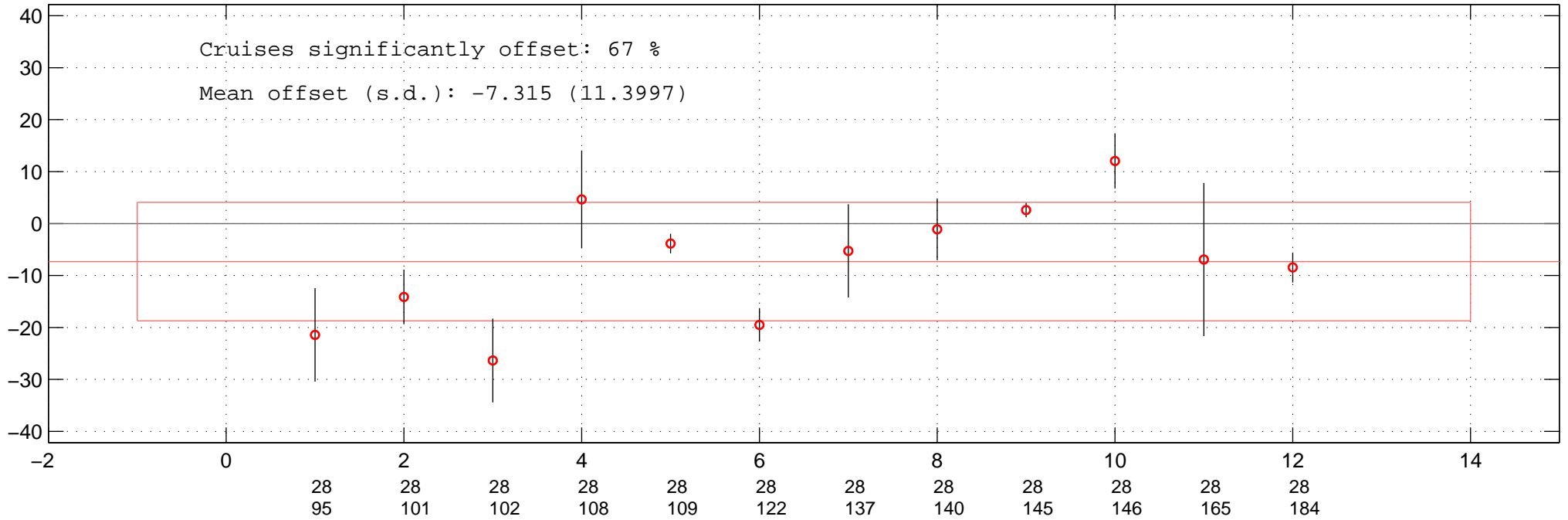
Additive offsets for ALK for 06MT19921227 in Favourite-space.
