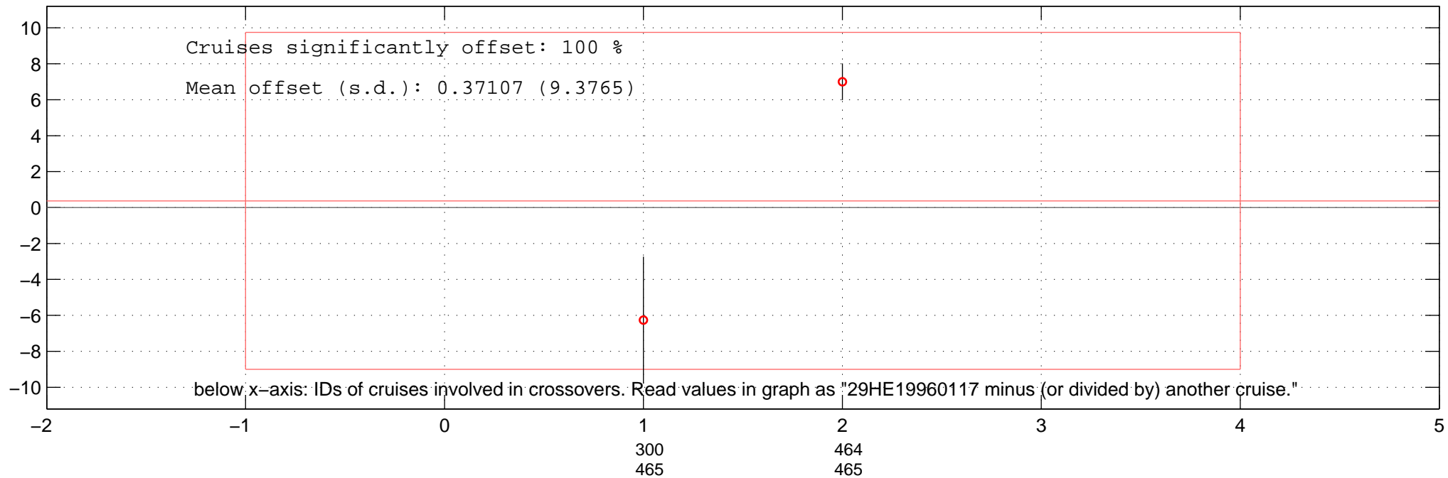
all additive offsets of ALK of 29HE19960117 in Favourite-space.
