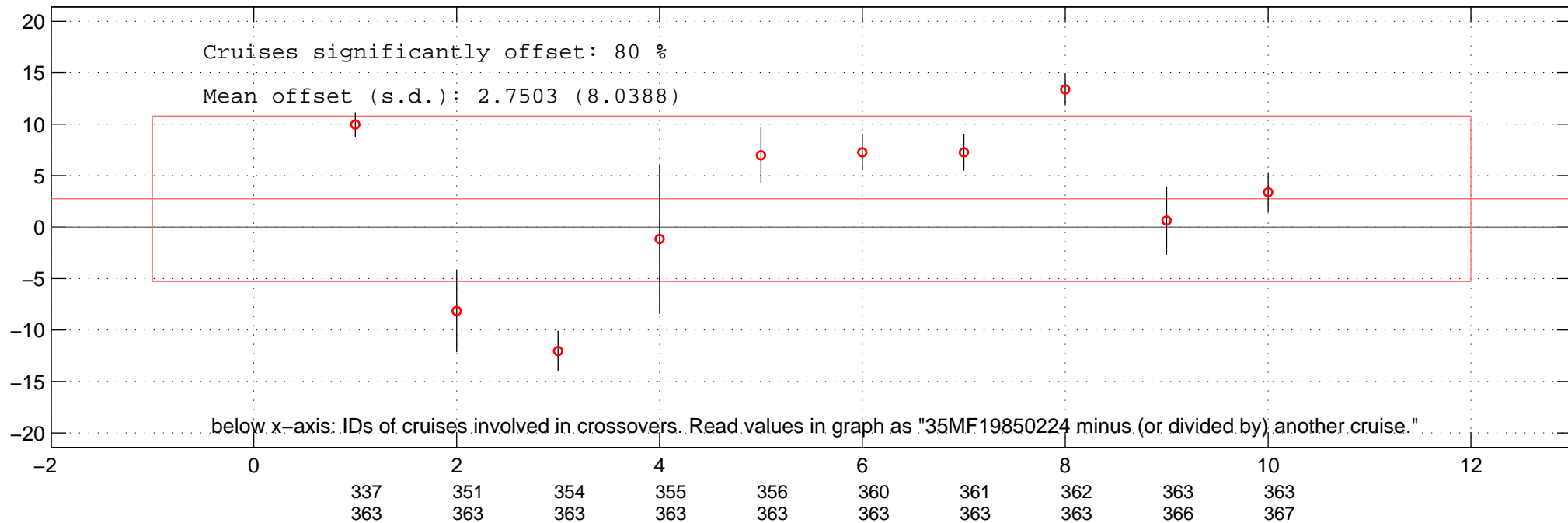
all additive offsets of ALK of 35MF19850224 in Favourite-space.
