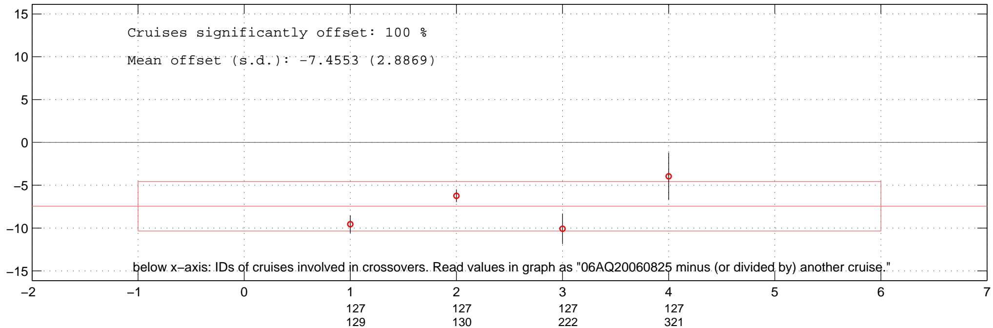
all additive offsets of ALK of 06AQ20060825 in Favourite-space.
