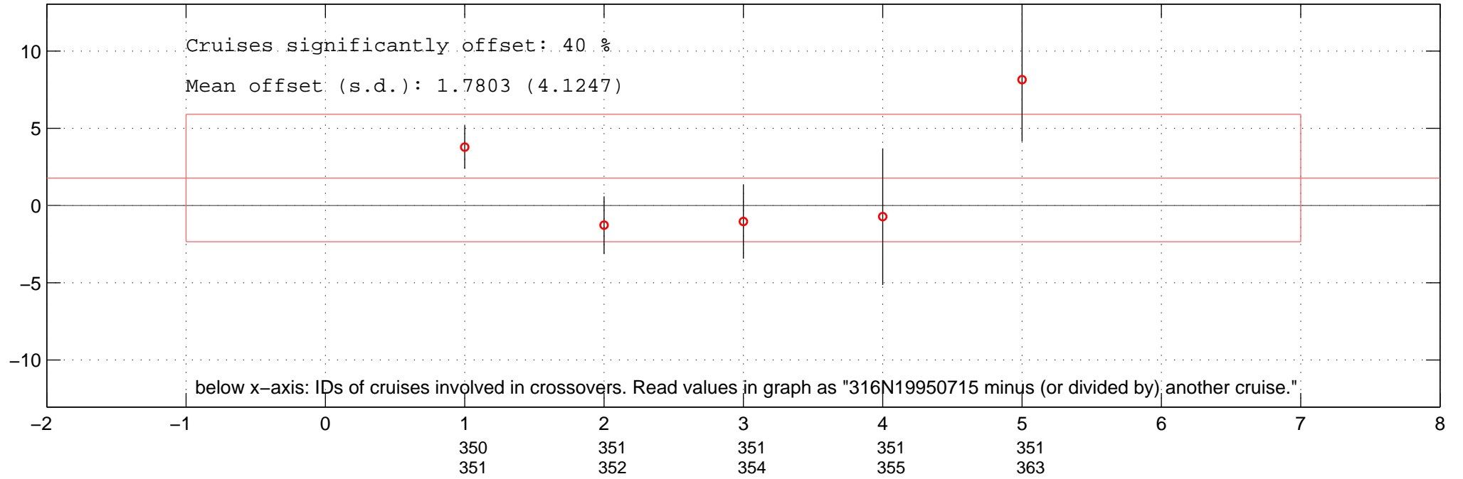
all additive offsets of ALK of 316N19950715 in Favourite-space.
