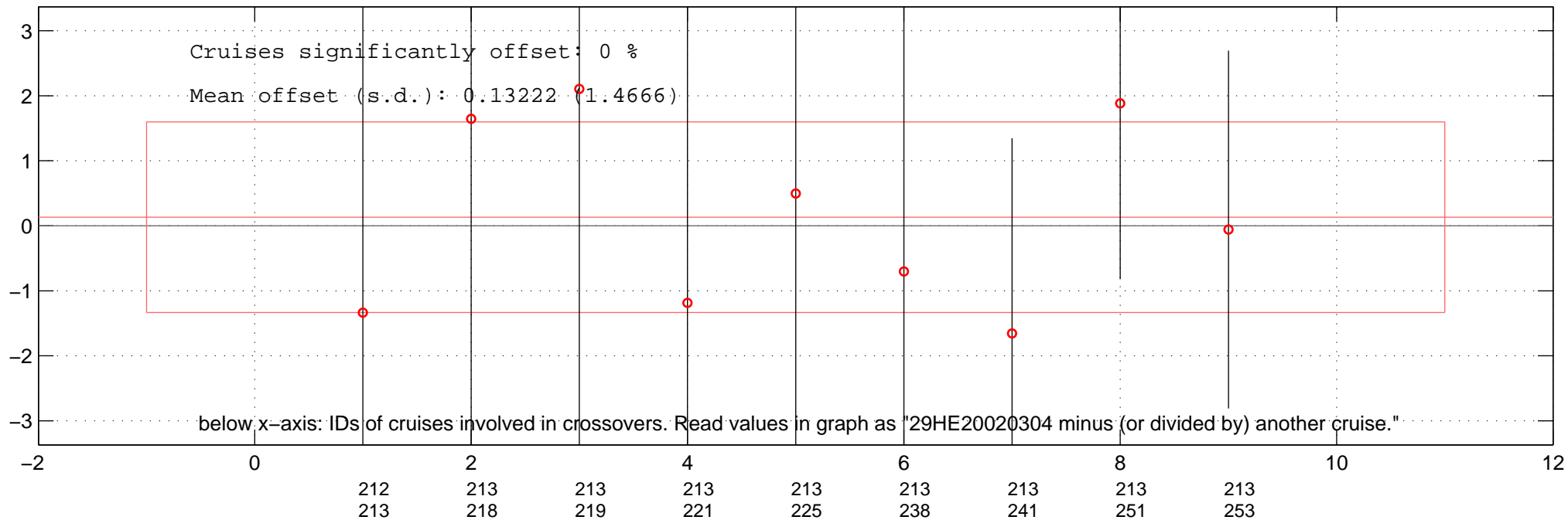
all multiplicative offsets of NO3 of 29HE20020304 in Favourite-space.
