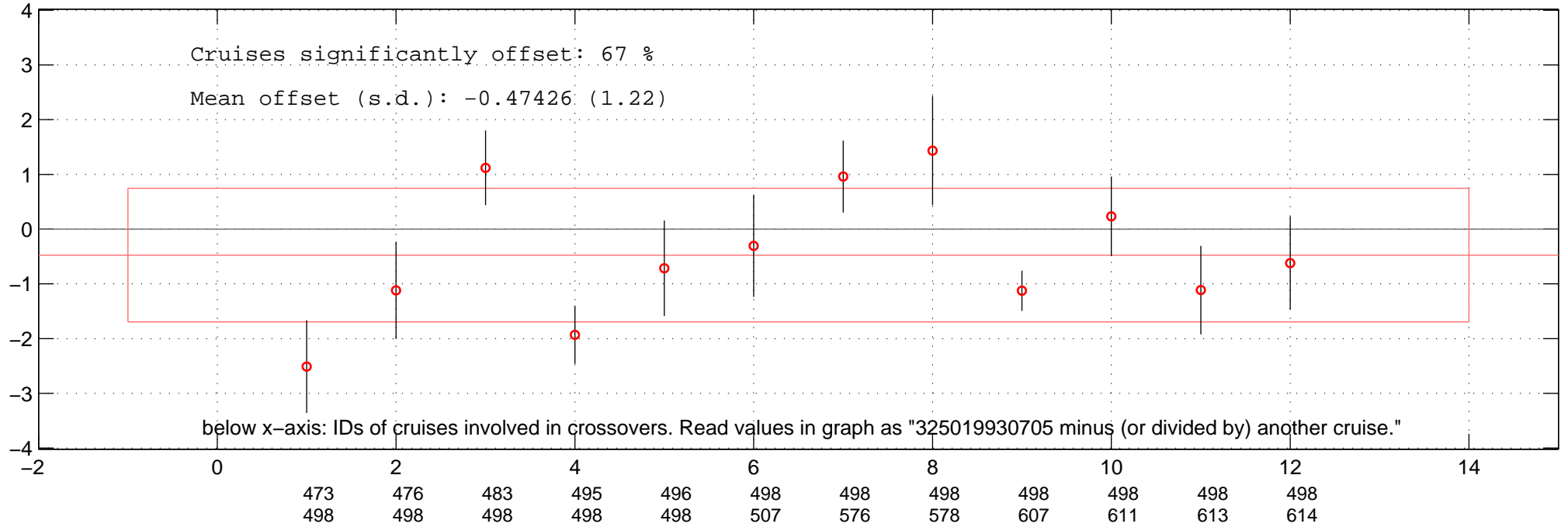
all multiplicative offsets of NO3 of 325019930705 in Favourite-space.
