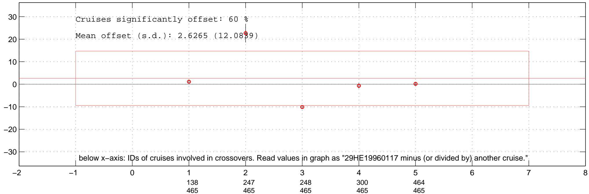
all multiplicative offsets of NO3 of 29HE19960117 in Favourite-space.
