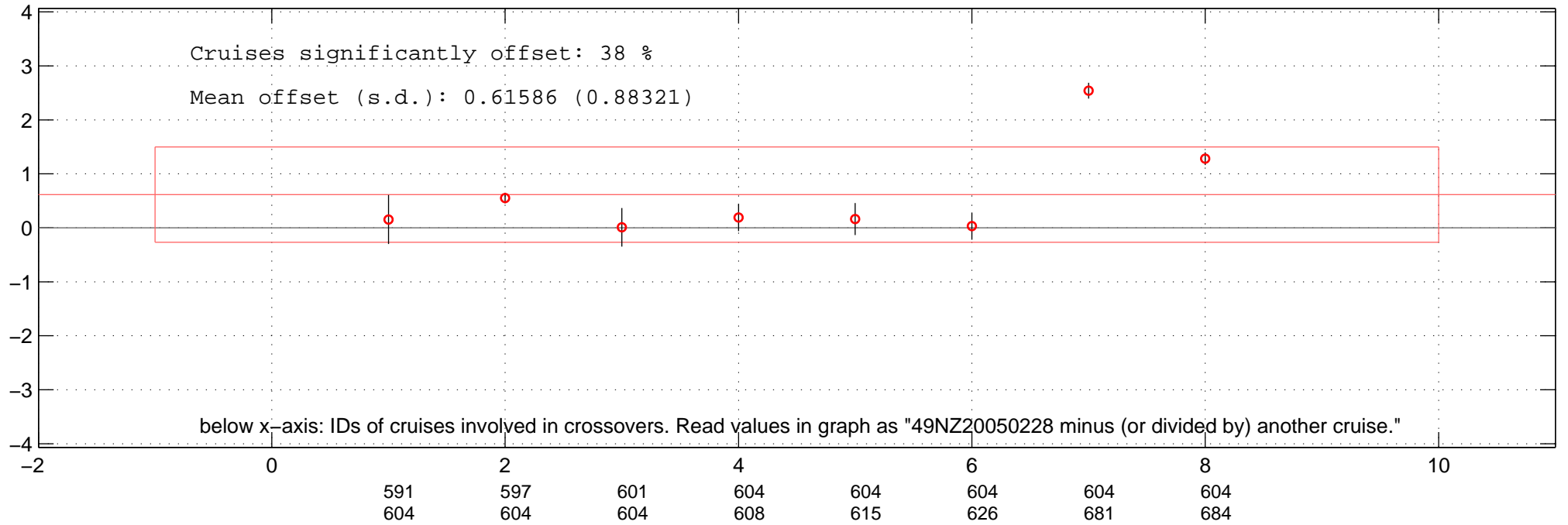
all multiplicative offsets of NO3 of 49NZ20050228 in Favourite-space.
