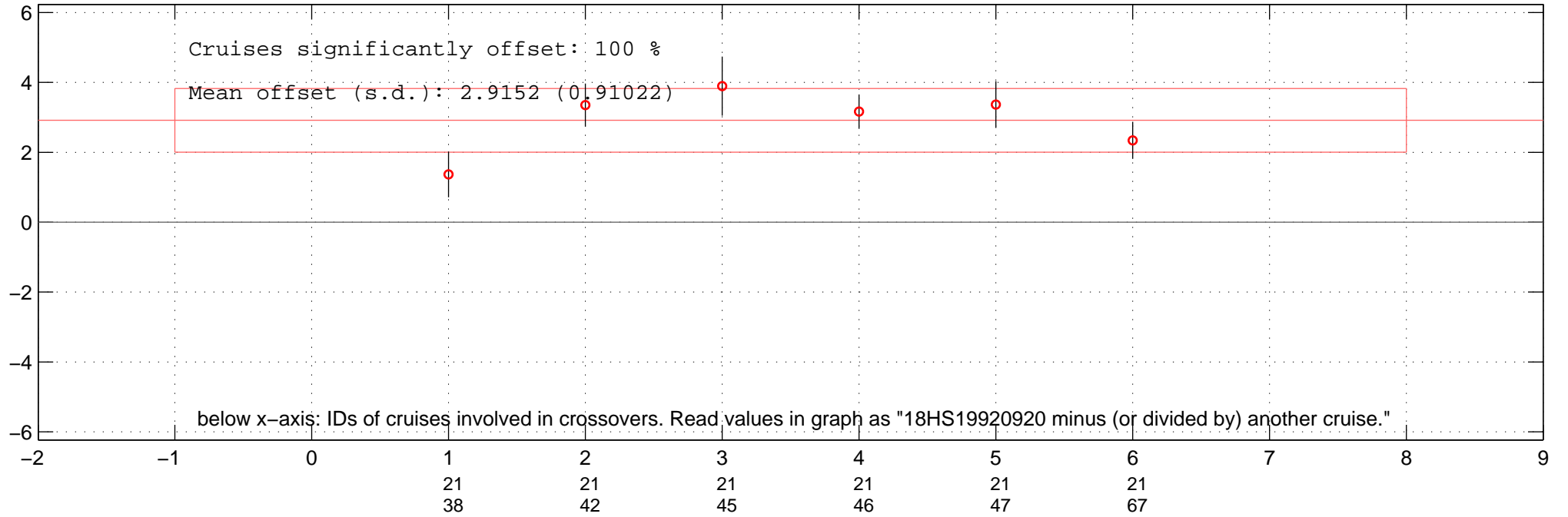
all multiplicative offsets of NO3 of 18HS19920920 in Favourite-space.
