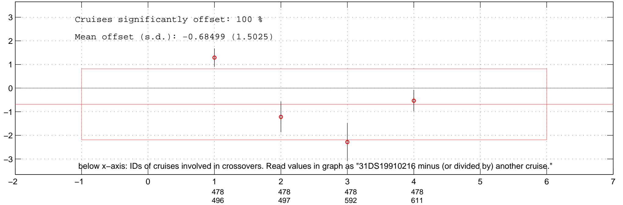
all multiplicative offsets of NO3 of 31DS19910216 in Favourite-space.
