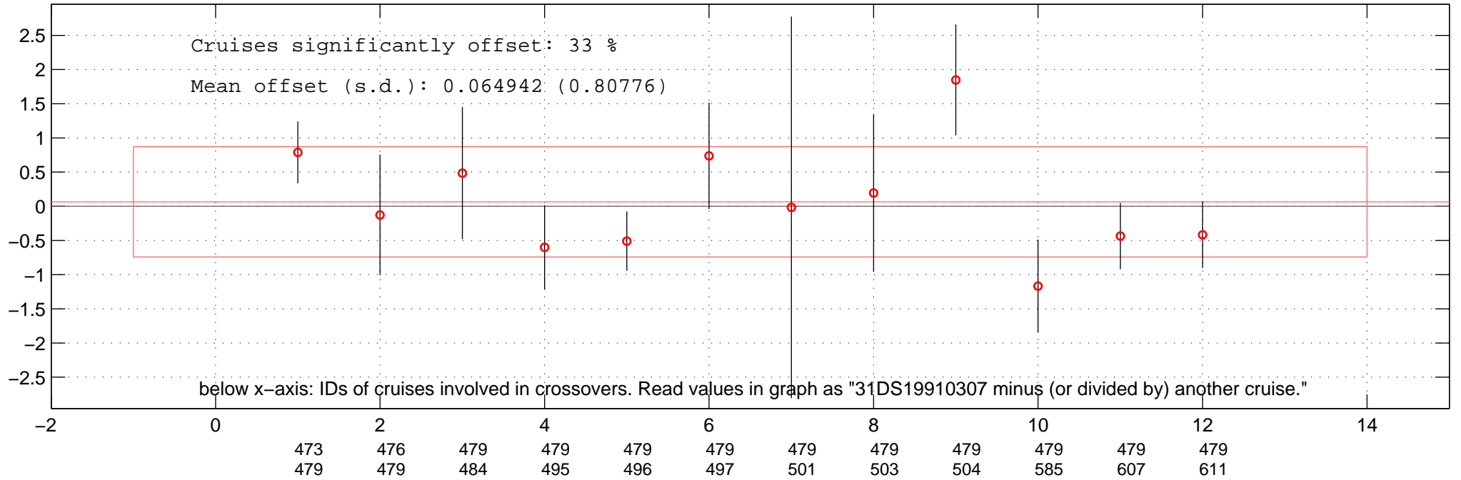
all multiplicative offsets of NO3 of 31DS19910307 in Favourite-space.
