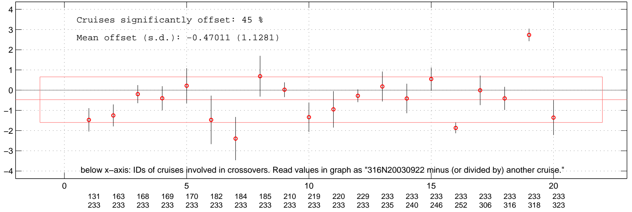
all multiplicative offsets of O2 of 316N20030922 in Favourite-space.
