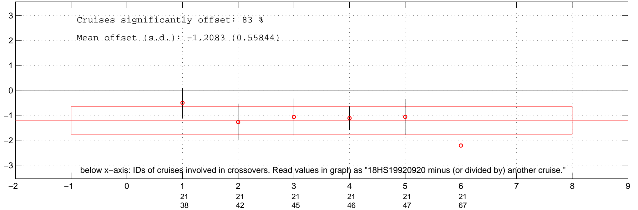
all multiplicative offsets of O2 of 18HS19920920 in Favourite-space.
