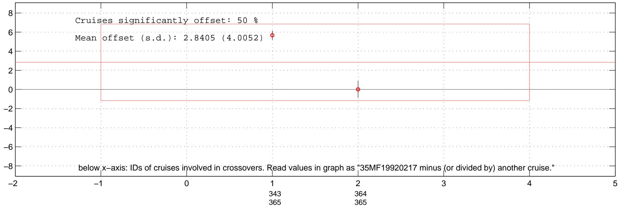
all multiplicative offsets of O2 of 35MF19920217 in Favourite-space.
