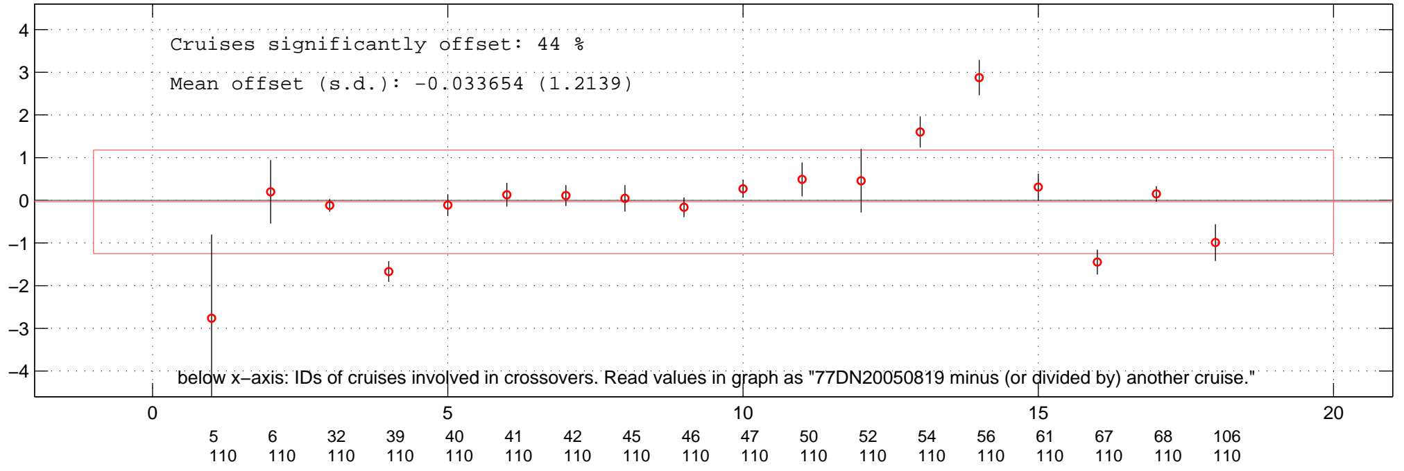
all multiplicative offsets of O2 of 77DN20050819 in Favourite-space.
