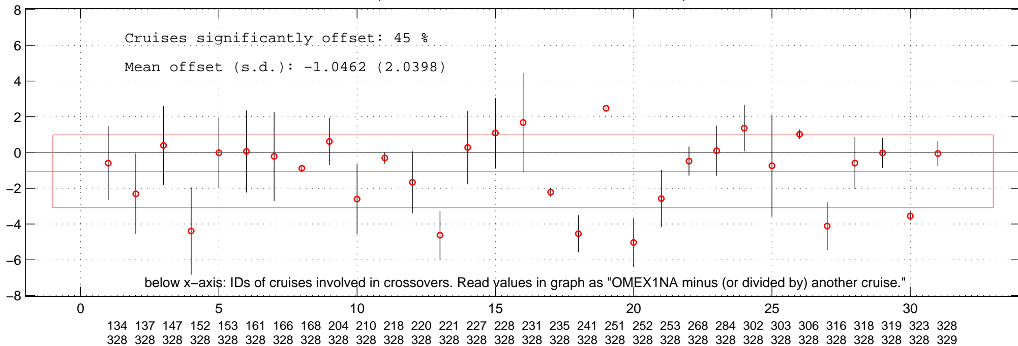
all multiplicative offsets of O2 of OMEX1NA in Favourite-space.
