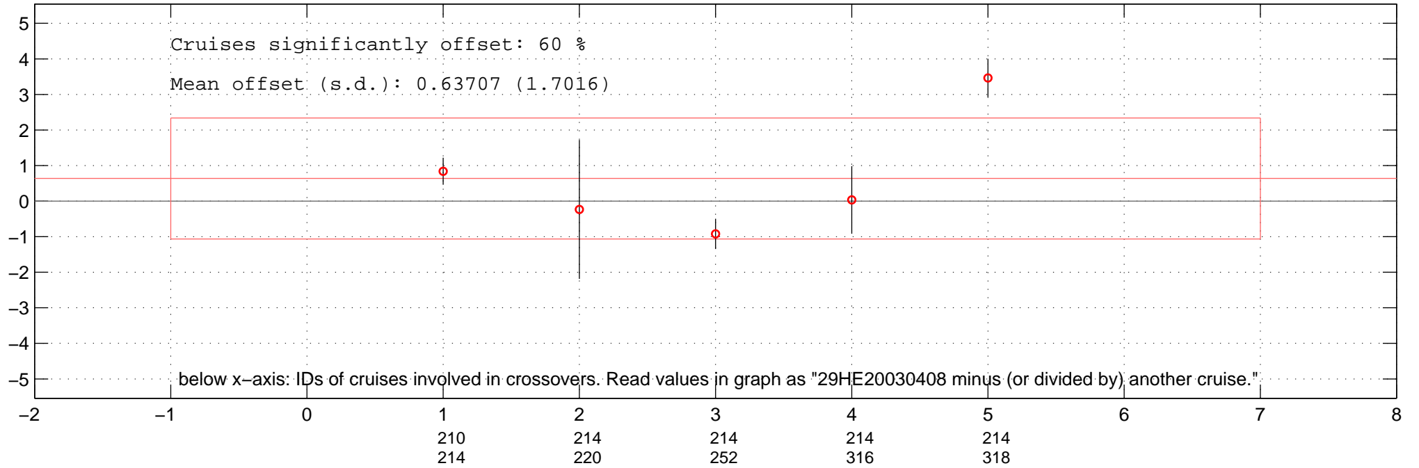
all multiplicative offsets of O2 of 29HE20030408 in Favourite-space.
