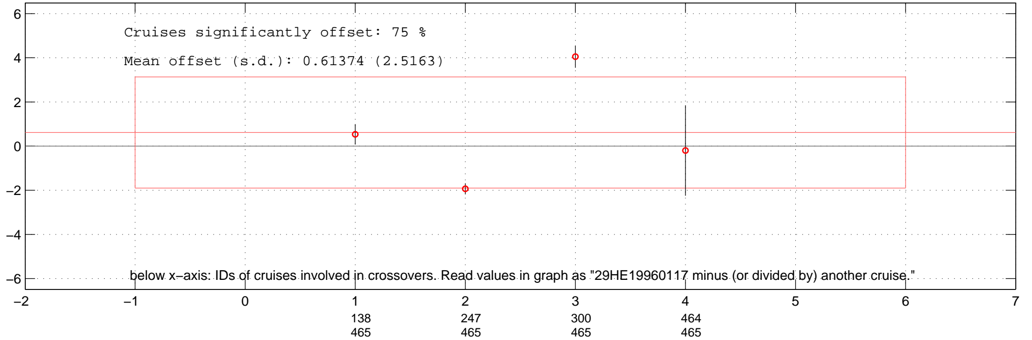
all multiplicative offsets of O2 of 29HE19960117 in Favourite-space.
