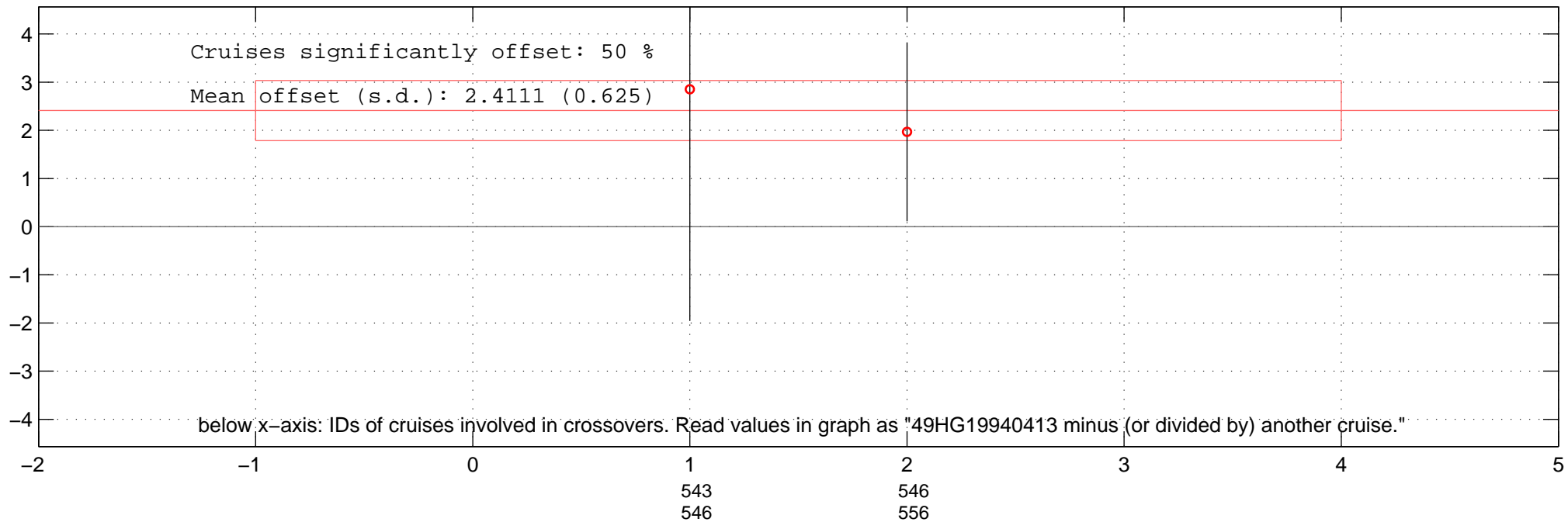
all multiplicative offsets of O2 of 49HG19940413 in Favourite-space.
