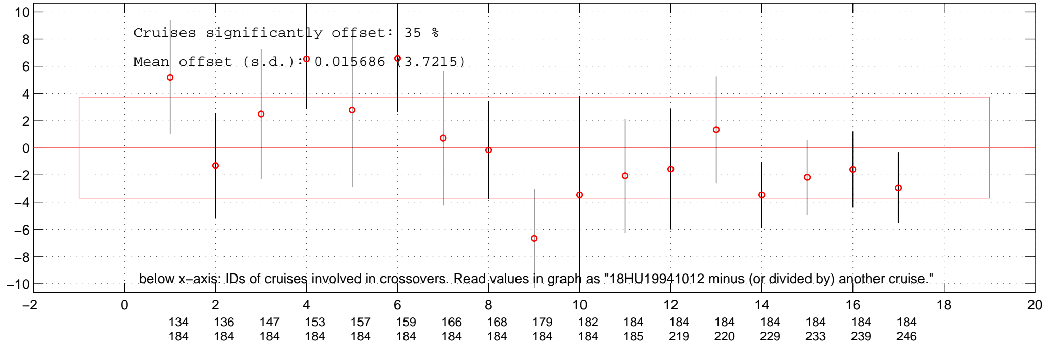
all multiplicative offsets of PO4 of 18HU19941012 in Favourite-space.
