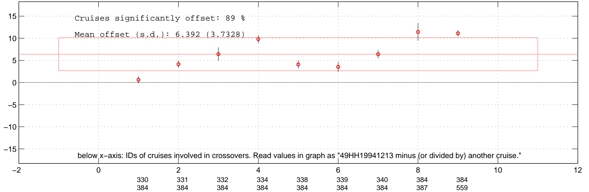
all multiplicative offsets of PO4 of 49HH19941213 in Favourite-space.
