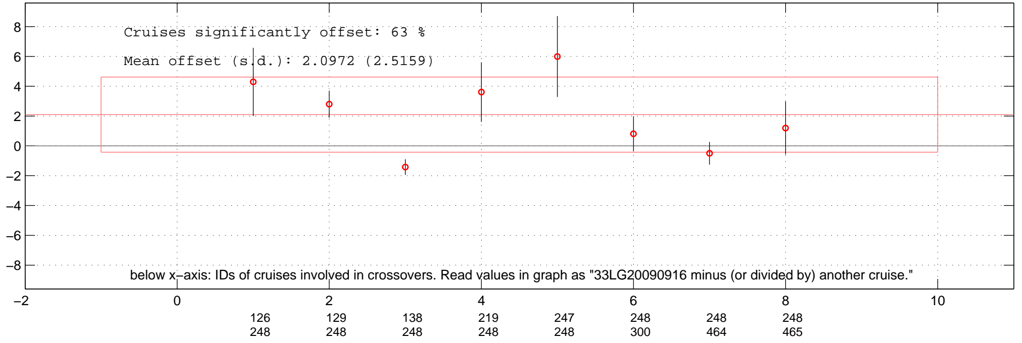
all multiplicative offsets of PO4 of 33LG20090916 in Favourite-space.
