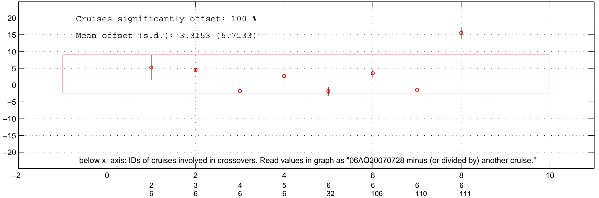
all multiplicative offsets of PO4 of 06AQ20070728 in Favourite-space.
