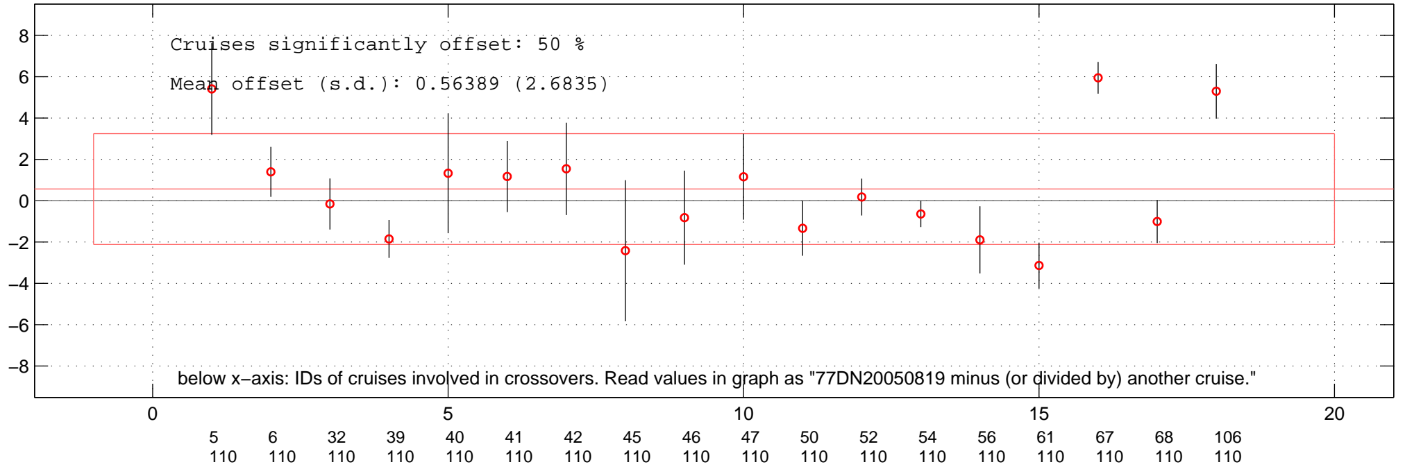
all multiplicative offsets of PO4 of 77DN20050819 in Favourite-space.
