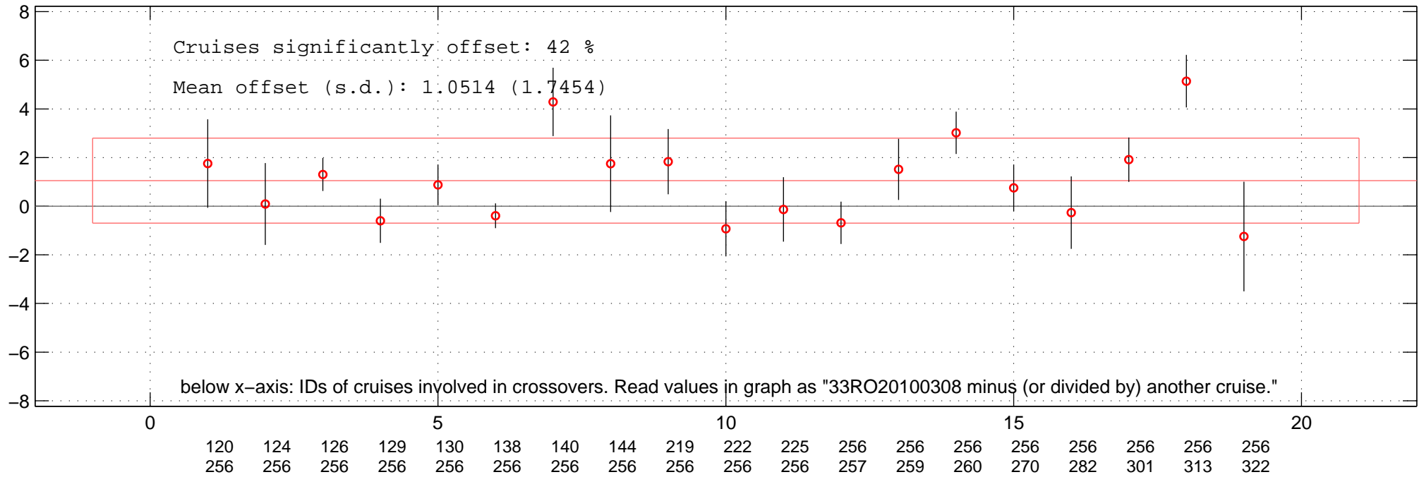
all multiplicative offsets of PO4 of 33RO20100308 in Favourite-space.
