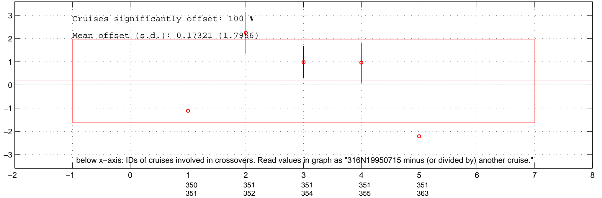
all multiplicative offsets of PO4 of 316N19950715 in Favourite-space.
