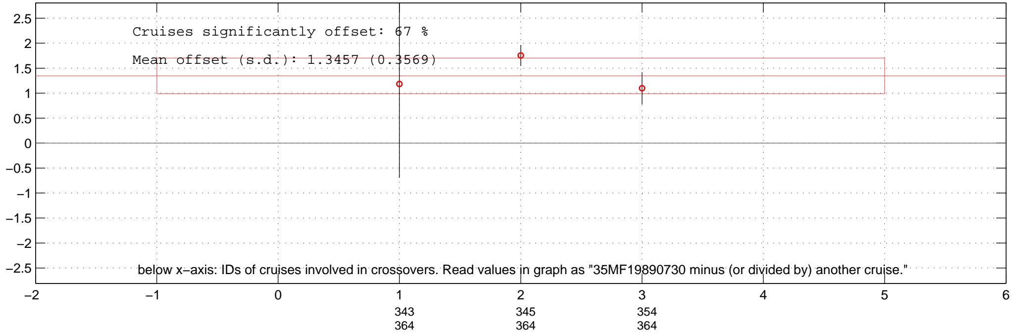
all multiplicative offsets of PO4 of 35MF19890730 in Favourite-space.
