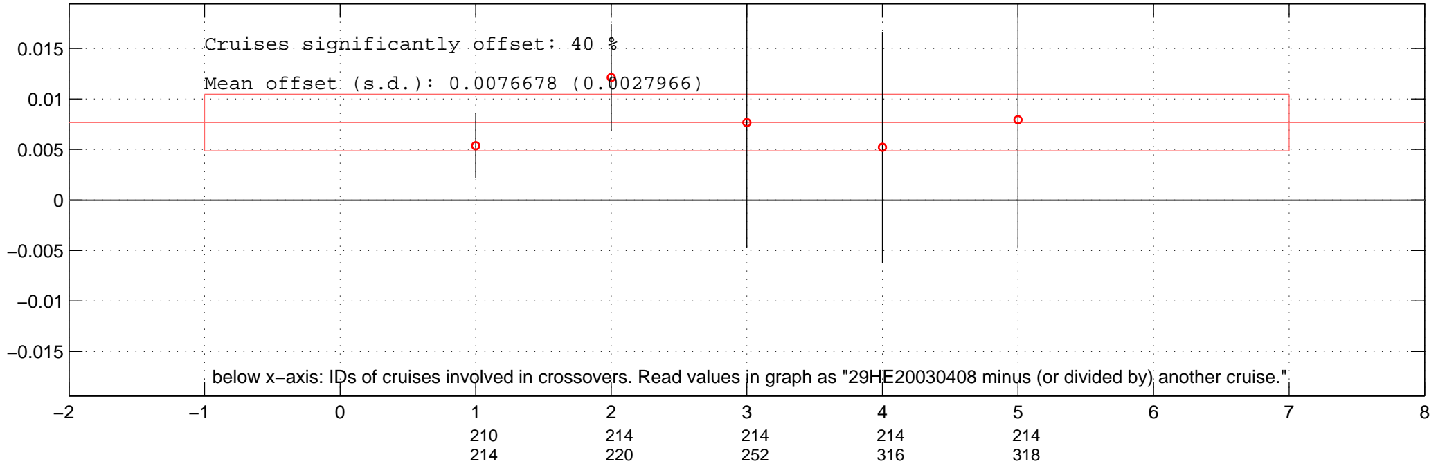
all additive offsets of SAL of 29HE20030408 in Favourite-space.
