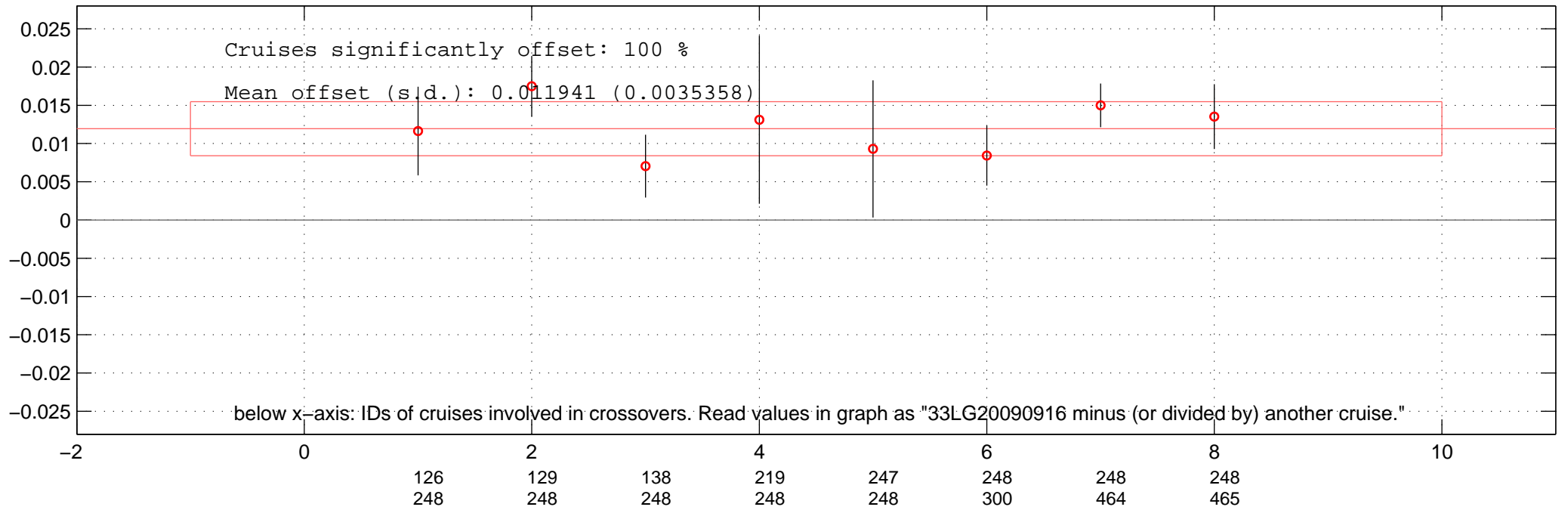
all additive offsets of SAL of 33LG20090916 in Favourite-space.
