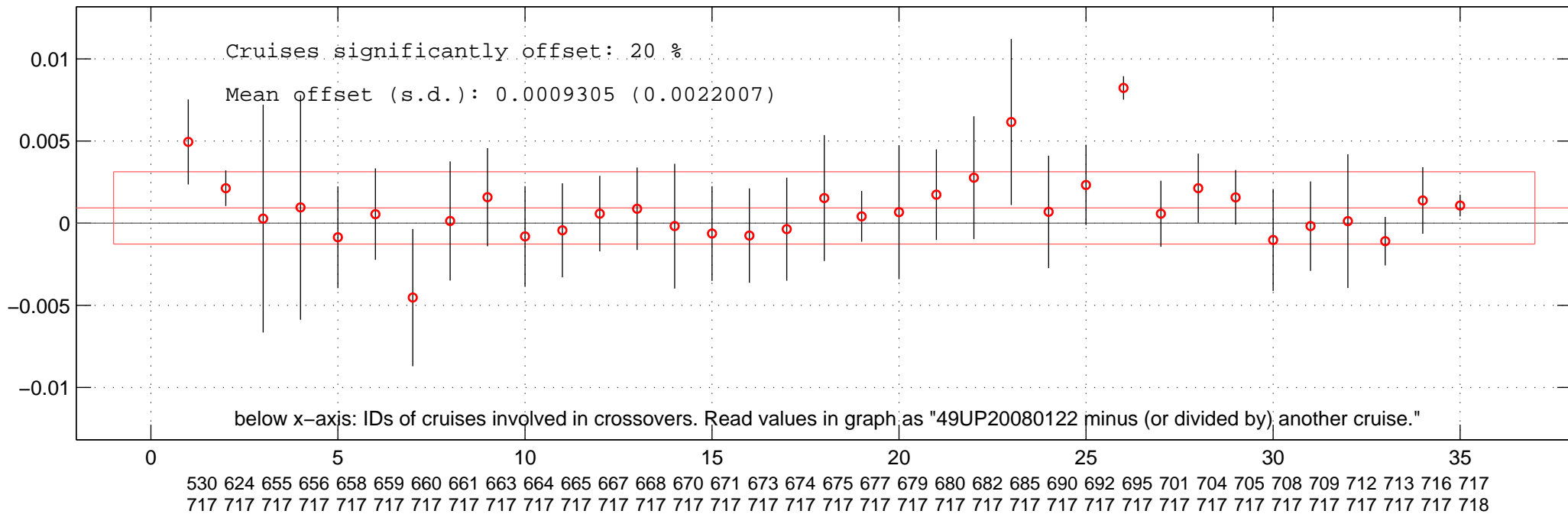
all additive offsets of SAL of 49UP20080122 in Favourite-space.
