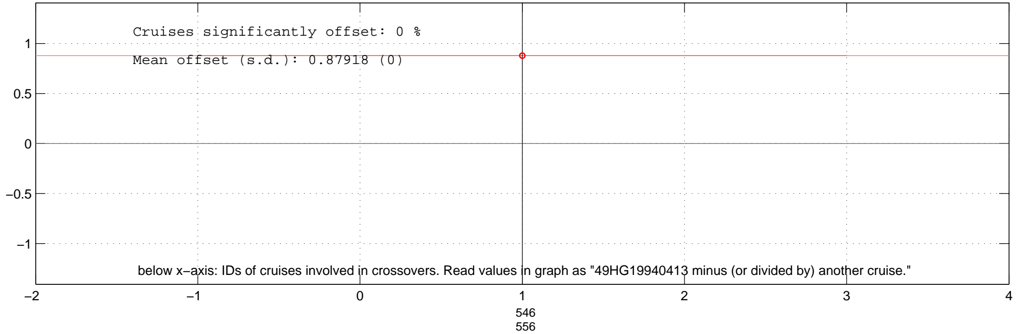
all multiplicative offsets of SIL of 49HG19940413 in Favourite-space.
