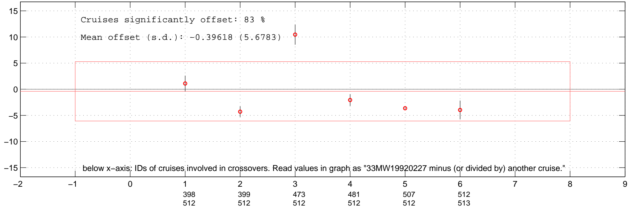
all multiplicative offsets of SIL of 33MW19920227 in Favourite-space.
