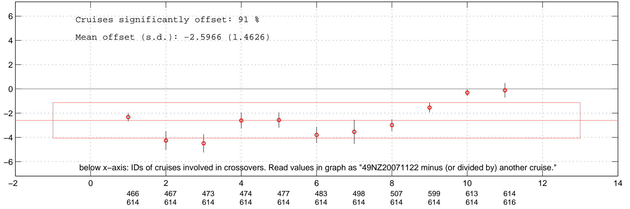
all multiplicative offsets of SIL of 49NZ20071122 in Favourite-space.
