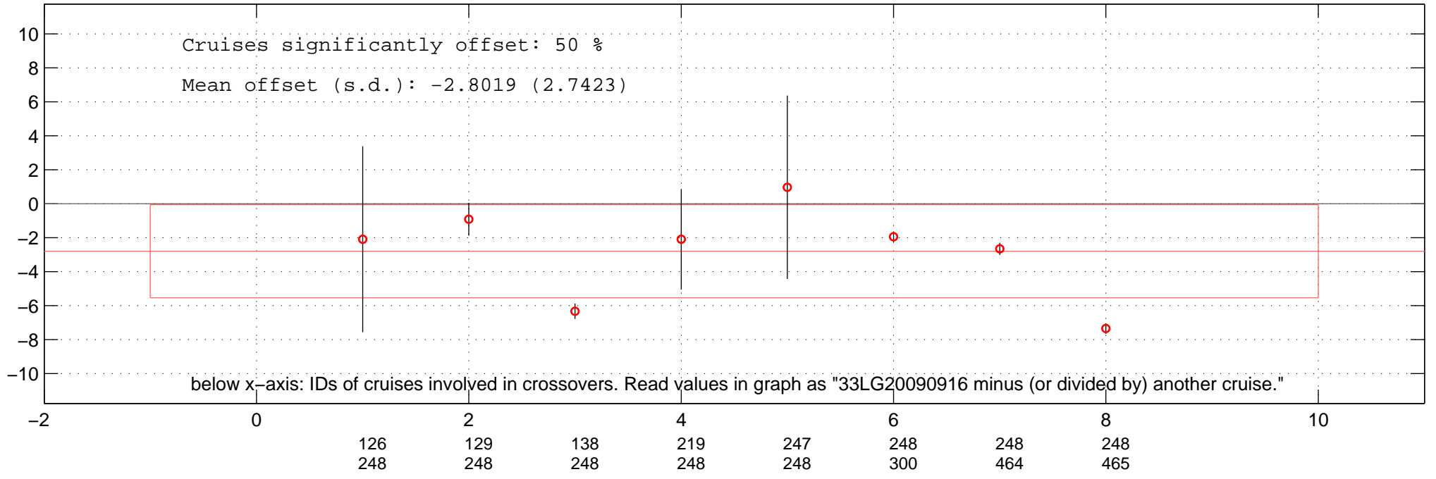
all multiplicative offsets of SIL of 33LG20090916 in Favourite-space.
