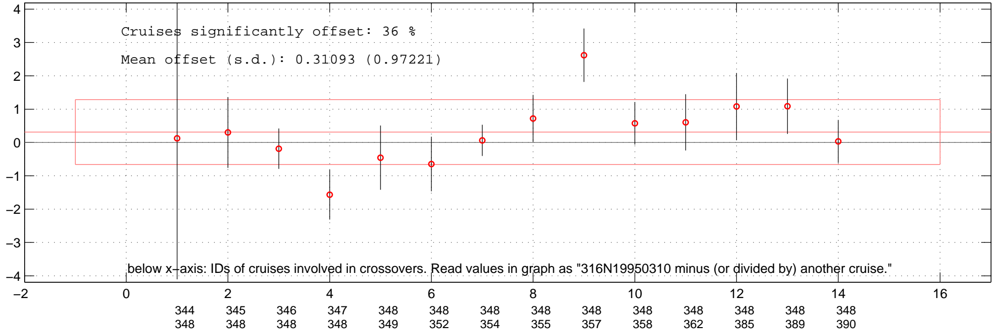
all multiplicative offsets of SIL of 316N19950310 in Favourite-space.
