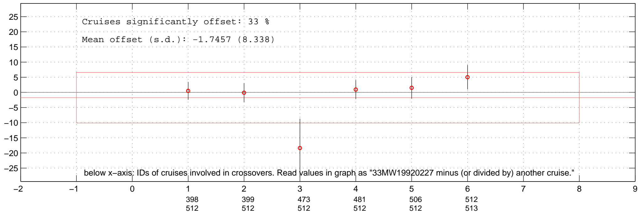
all additive offsets of DIC of 33MW19920227 in Favourite-space.
