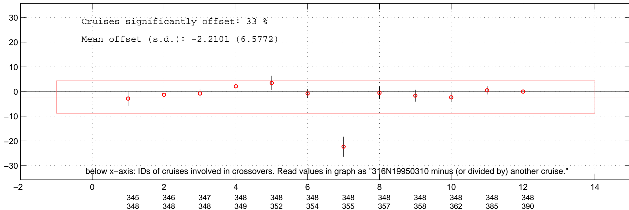
all additive offsets of DIC of 316N19950310 in Favourite-space.
