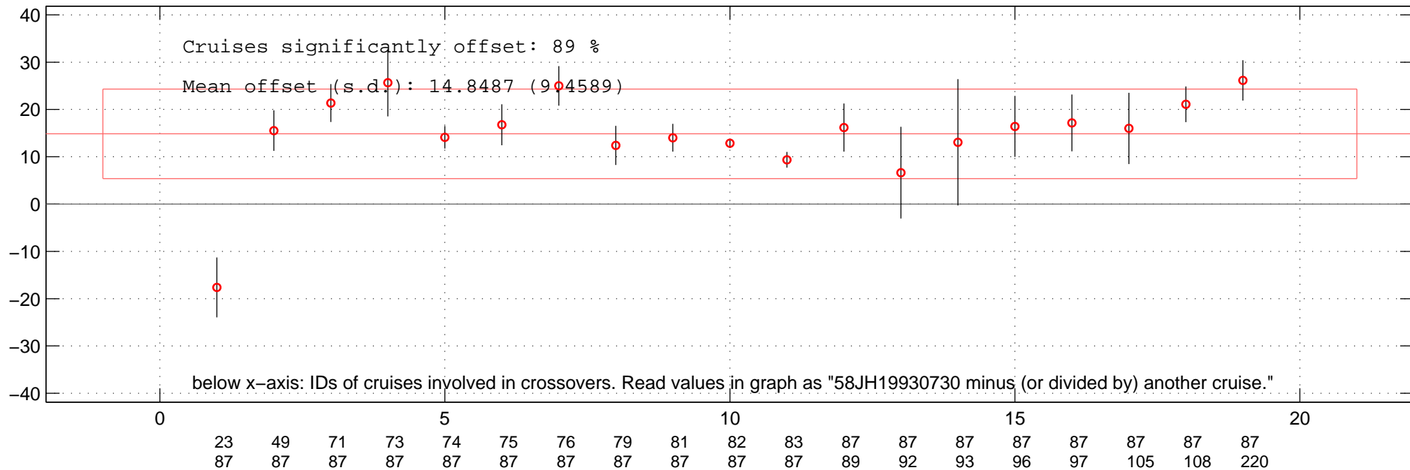
all additive offsets of DIC of 58JH19930730 in Favourite-space.
