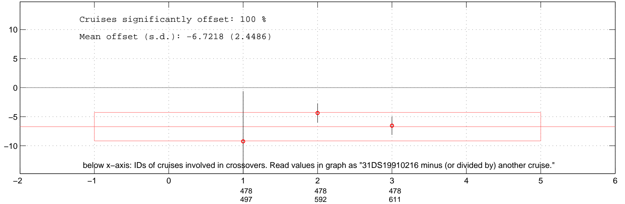
all additive offsets of DIC of 31DS19910216 in Favourite-space.
