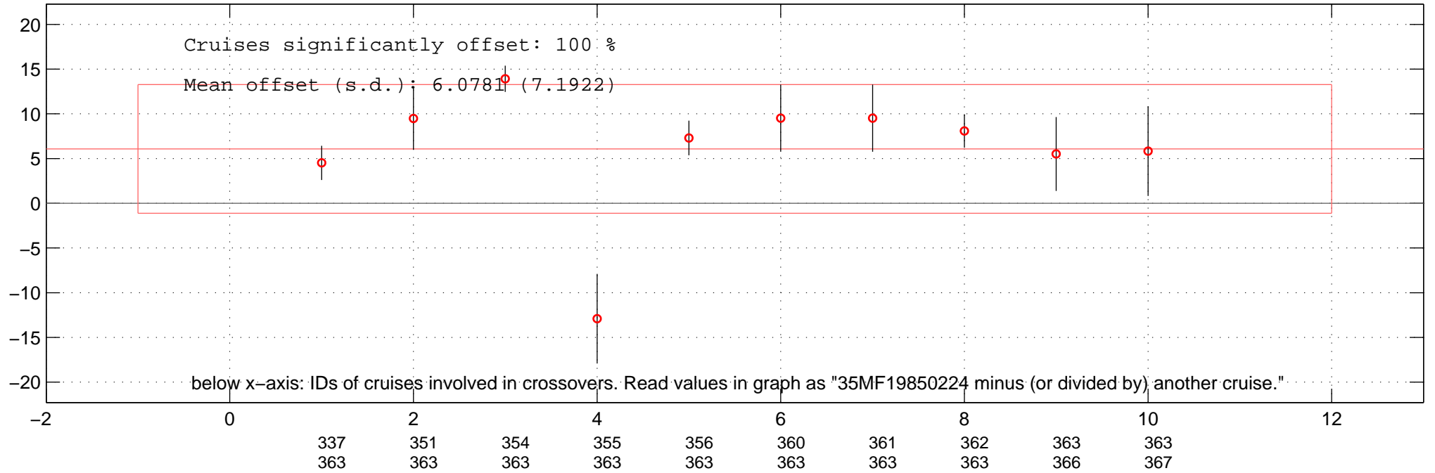
all additive offsets of DIC of 35MF19850224 in Favourite-space.
