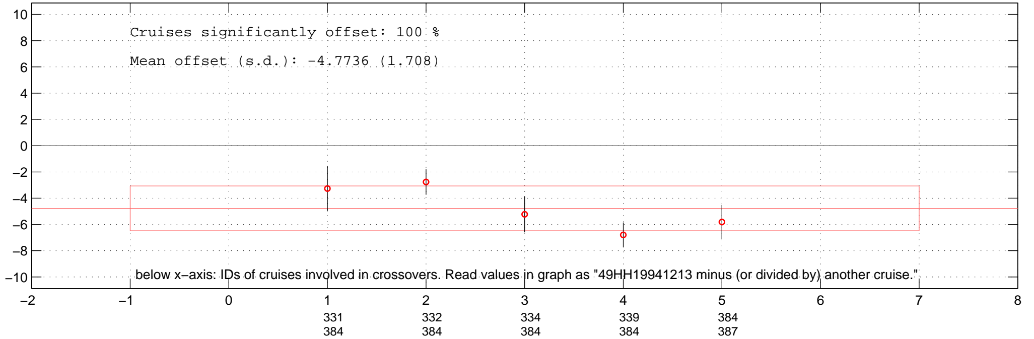
all additive offsets of DIC of 49HH19941213 in Favourite-space.
