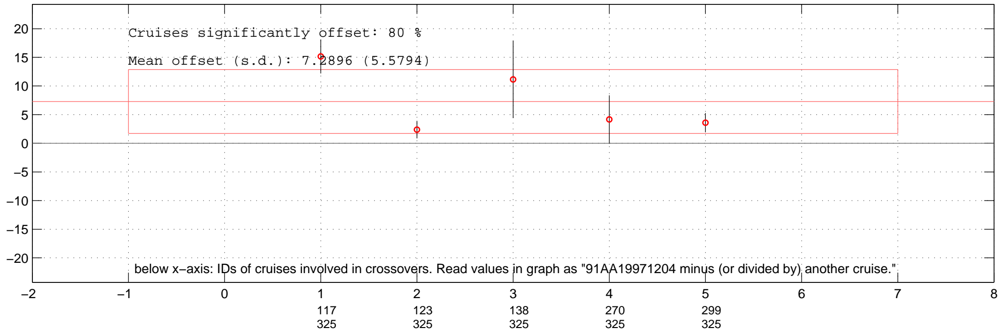
all additive offsets of DIC of 91AA19971204 in Favourite-space.
