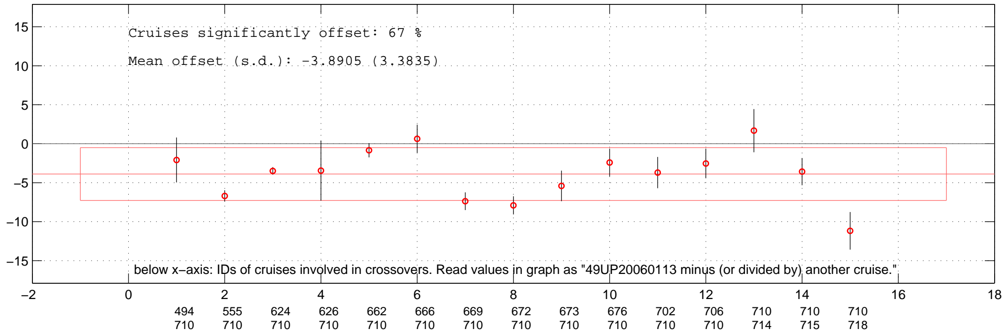
all additive offsets of DIC of 49UP20060113 in Favourite-space.
