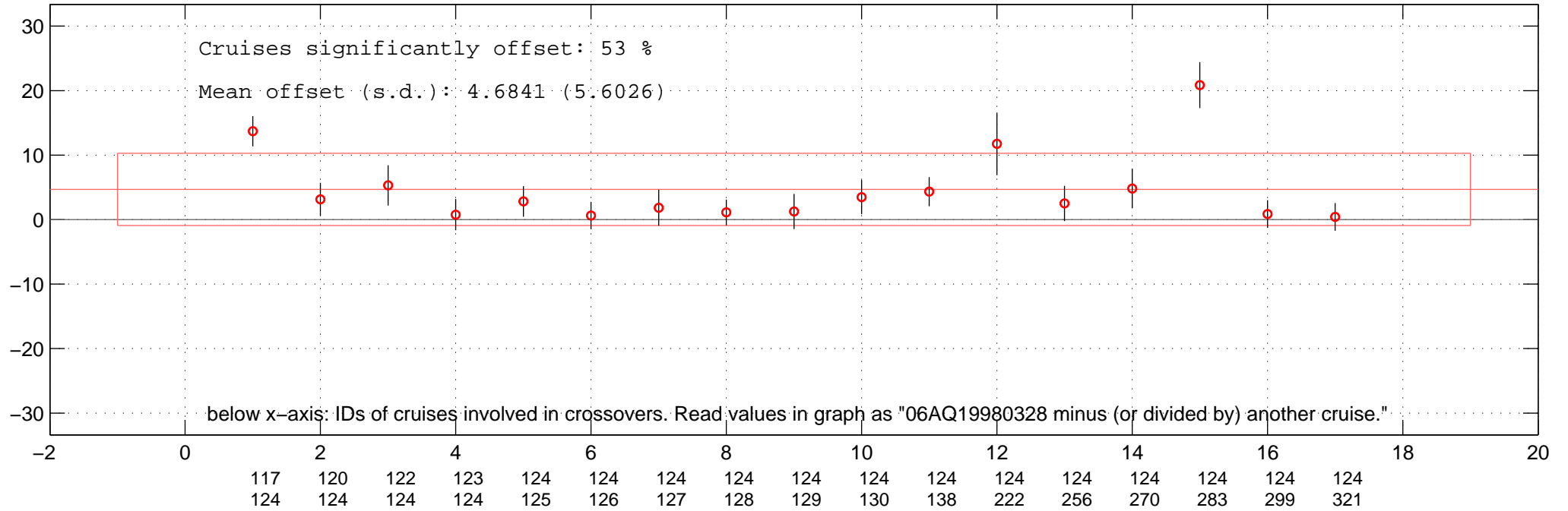
all additive offsets of DIC of 06AQ19980328 in Favourite-space.
